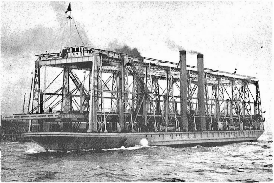
▲ THE TRAIN-FERRY S.S. LEONARD UNDERGOING HER SPEED TRIALS IN THE ESTUARY of the Mersey River, off Birkenhead and Liverpool in August, 1914. This photograph appeared in a history of Messrs. Cammell Laird and Company and is reproduced with their kind permission.
