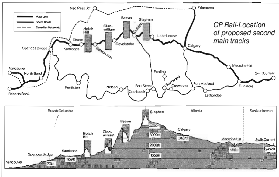
Double tracking: Diagram shows location of proposed improvements to the mainline. The project is scheduled for completion by 1980.
