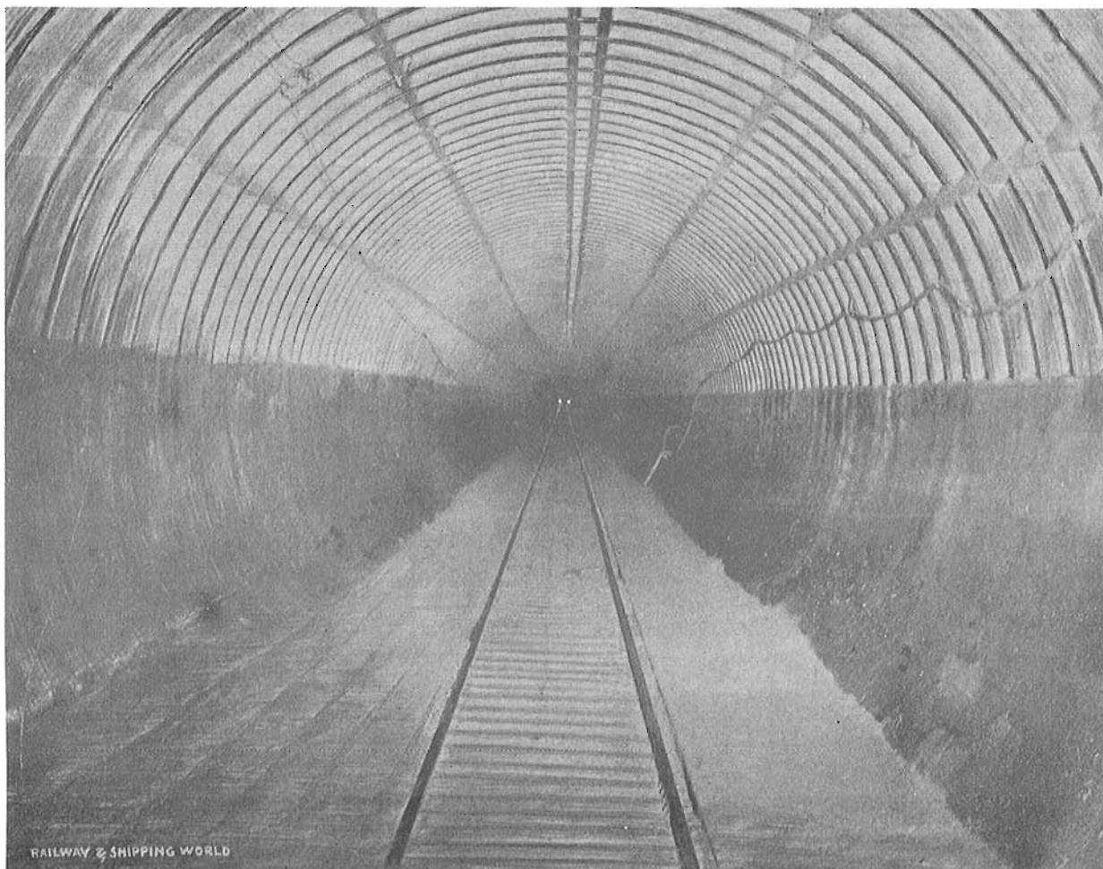
This flash-illuminated view of the interior of the St. Clair tunnel was taken, in 1899, as part of the successful project to photograph, by motion picture camera, the entire bore of the tunnel from portal to portal. Since the view was taken only eight years after the tunnel went into service, it shows it essentially as built.
