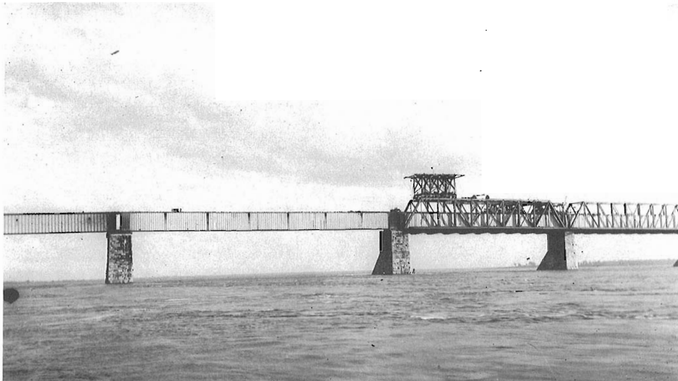
While no photo of the rebuilding of the Ste. Annes bridge has so far come to light, the method was likely similar to the way the Victoria Bridge was rebuilt at about the same time. This photo, taken from a boat on July 2, 1898, shows the new steelwork being built around the old tube. The latter was then removed with minimal interruption to traffic.
