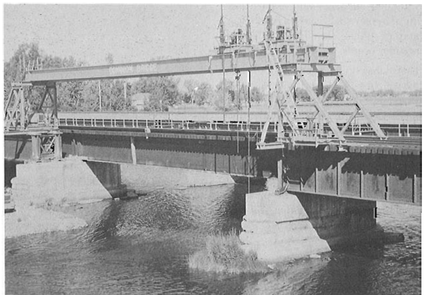
Installing new beam.
